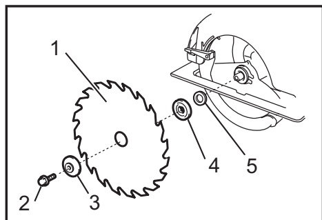
► 1. Saw blade 2. Hex bolt 3. Outer flange 4. Inner flange 5. Ring
